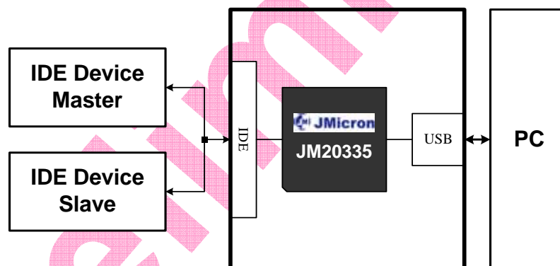
Fig. 2 Hi-Speed USB to PATA
